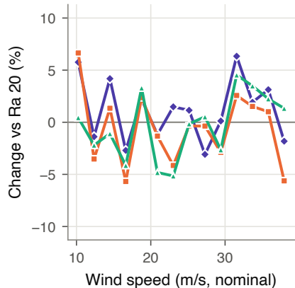
(c) R_{int} vs Ra 20
