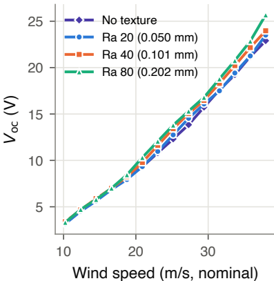
(a) Open-circuit voltage
