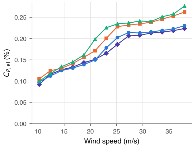
(b) Electrical power coefficient
