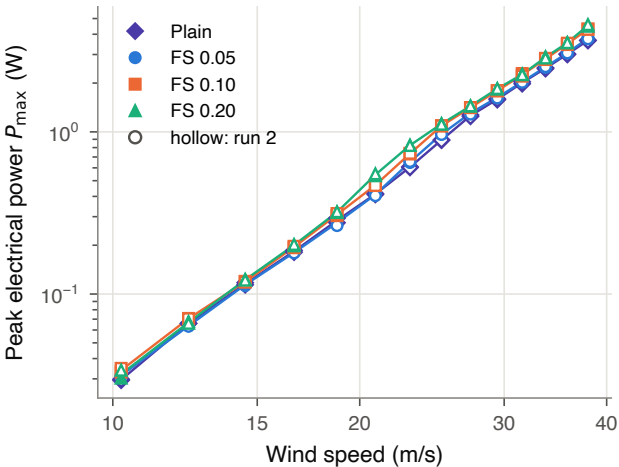
(a) Peak electrical power
