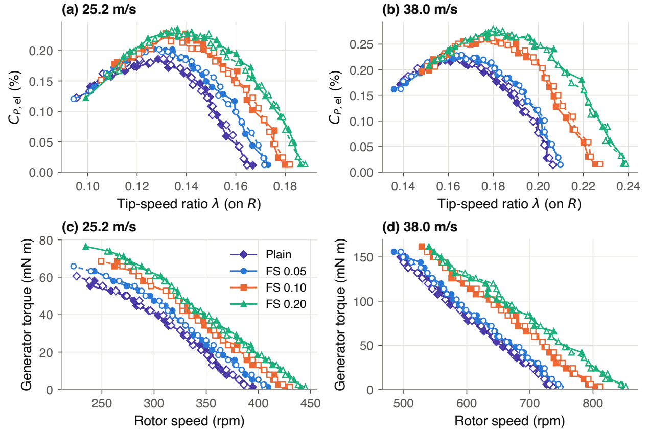
Figure 7. Electrical power coefficient against tip-speed ratio (a, b) and generator torque k_T I ( k_T = 0.30 \text{ N m/A} ) against rotor speed (c, d), from the speed at every load step; all eight runs (solid: run 1; dashed, hollow: run 2).
