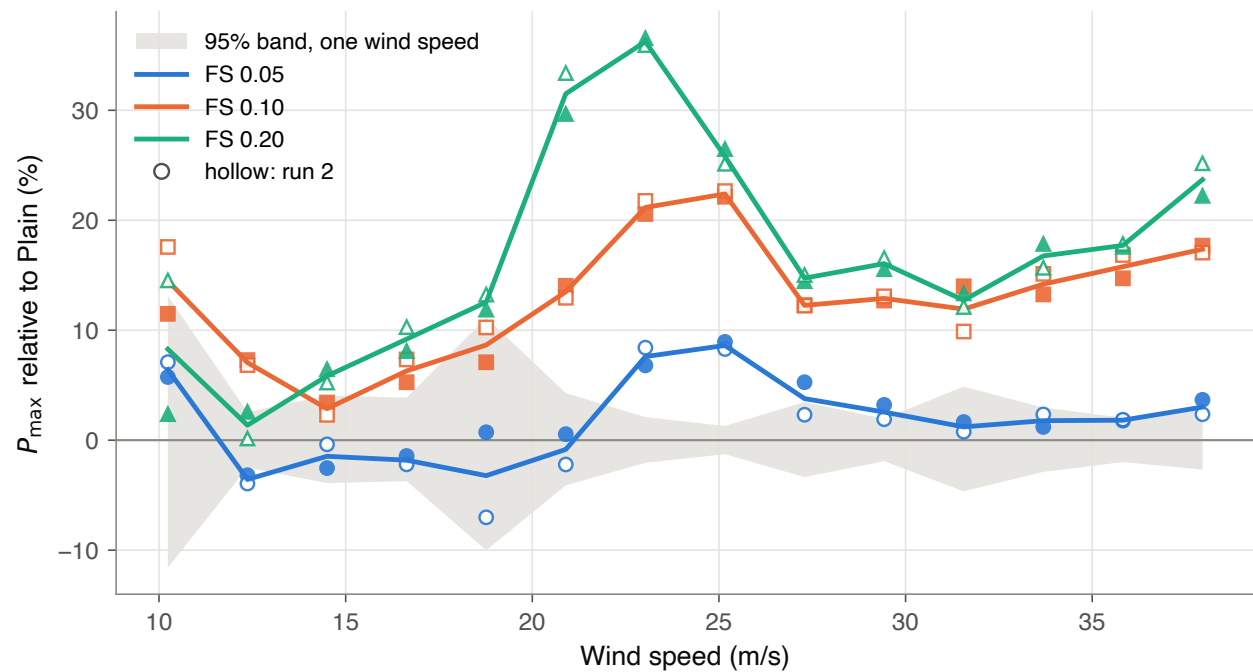
Figure 6. P_{\max} of each textured rotor relative to Plain at each wind speed. Markers: individual runs (filled: run 1; hollow: run 2); lines: geometric mean; band: 95% interval of a single-wind-speed difference from run-to-run scatter.
