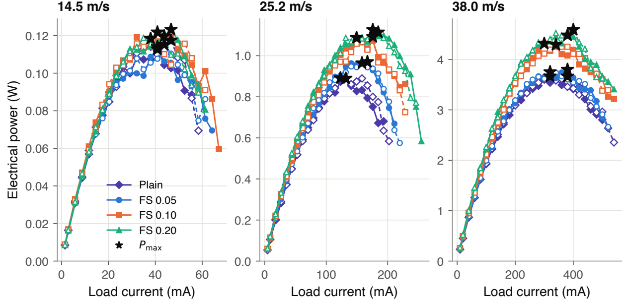
Figure 3. Measured load ladders at three wind speeds, all eight runs (solid: run 1; dashed, hollow: run 2). Stars mark P_{\max} , the largest dwell power.
