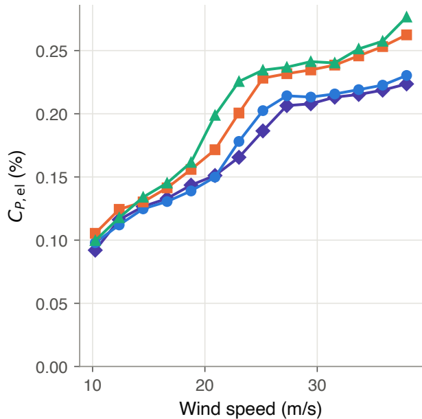
(b) Electrical power coefficient
