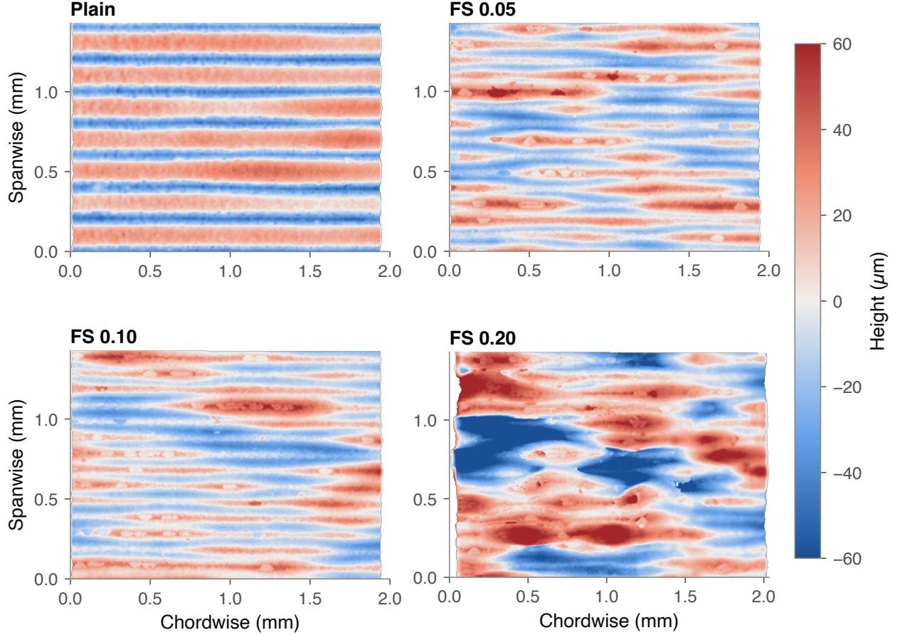
Figure 1. Profilometer height maps, one field per blade set, each column levelled. Layer lines run horizontally (chordwise); the Pa and Ra profiles run vertically (spanwise). Colour is clipped at \pm 60 \mu\text{m} , which FS 0.20 exceeds over 8% of its area.
