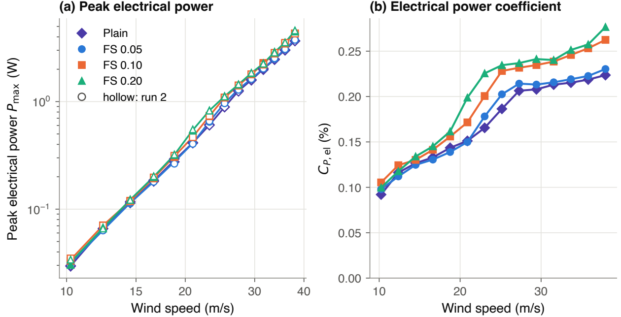
Figure 4. (a) Peak electrical power of every run on logarithmic axes (filled: run 1; hollow: run 2); lines join the geometric means of the two runs. (b) Electrical power coefficient, standard air density.
