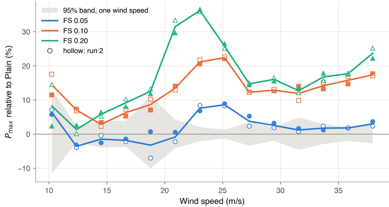
Figure 6. P_{\max} of each textured rotor relative to the Plain rotor at each wind speed. Markers: individual runs (filled: run 1; hollow: run 2); lines: geometric mean of the two runs; band: 95% interval of a single-wind-speed difference from run-to-run scatter. All curves share the Plain reference, so features common to all three may come from it.
