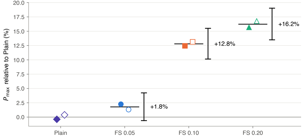
Figure 5. Each run’s mean P_{\max} relative to the Plain rotor (filled: run 1; hollow: run 2). Bars: rotor mean with the Tukey simultaneous 95% interval for the difference from Plain.
