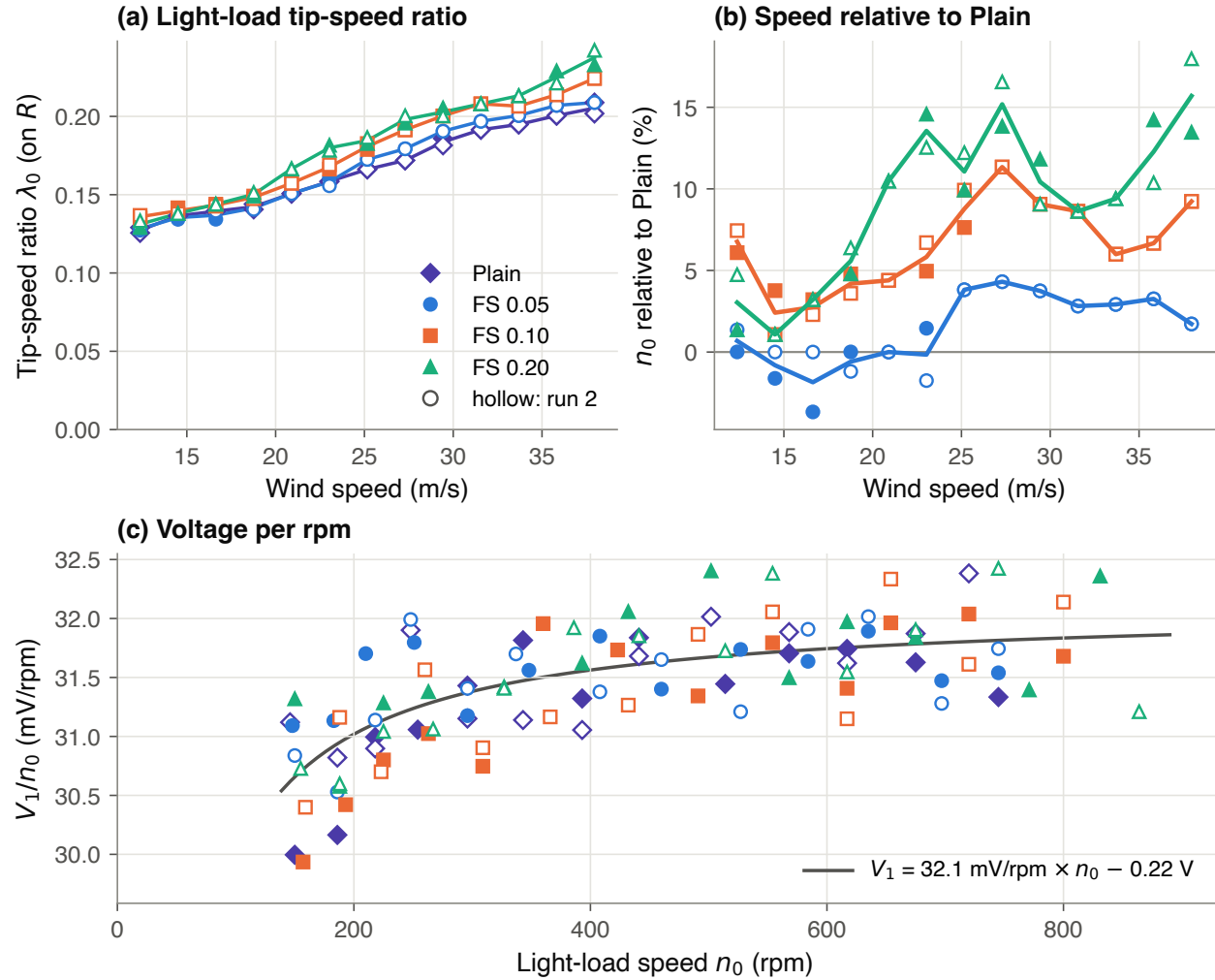
Figure 8. Light-load rotor speed n_0 from the tachometer at fan set points 600–1800 rpm (filled: run 1; hollow: run 2; lines: geometric mean of the two runs). (a) Tip-speed ratio \lambda_0 on the attachment radius. (b) n_0 of each textured rotor relative to Plain; one quantisation step is 0.7–4.0% of n_0 . (c) First-step voltage per rpm, V_1/n_0 , with the ratio implied by the least-squares line V_1 = a + bn_0 .
