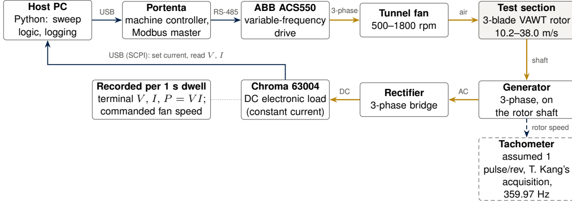
Figure 2. Measurement and control chain. The dashed path is T. Kang’s separate rotor-speed acquisition.
