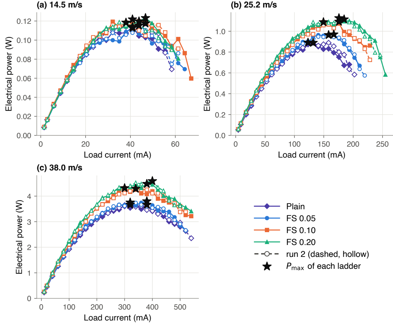
Figure 3. Measured load ladders at three wind speeds, all eight runs (solid: run 1; dashed, hollow: run 2). Stars mark P_{\max} , the largest dwell power.
