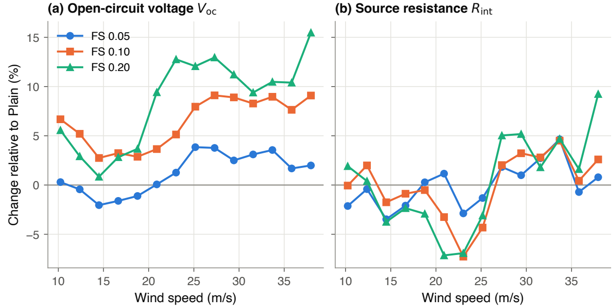
Figure 7. Thévenin parameters relative to the Plain rotor (geometric mean of two runs). (a) Extrapolated open-circuit voltage. (b) Apparent source resistance. All curves share the Plain reference, so features common to all three may come from it.
