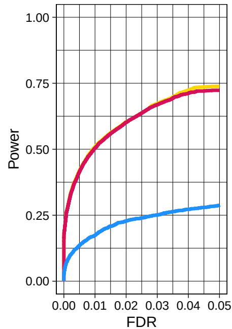
Wavelet GP noise
