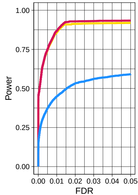
WGBS distance decay
