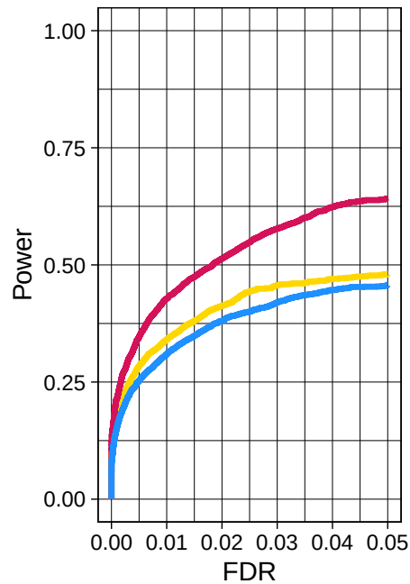
Wavelet fractional noise
