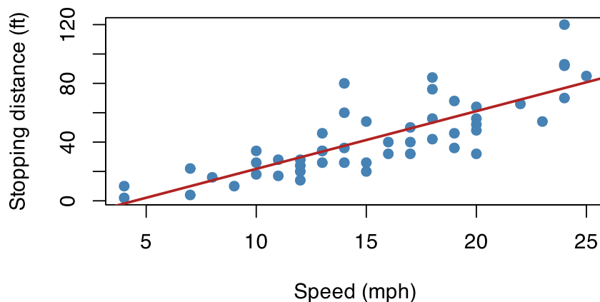
Figure 2: Stopping distance against speed for the built-in cars data, with a least-squares fit.
