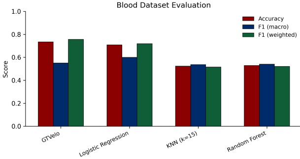
Fig. 1. Metric comparison across model on the blood lineage subset of the MOCA dataset.
