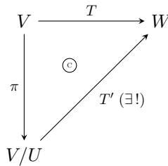
Figure 3: Map diagram of the map T' .
