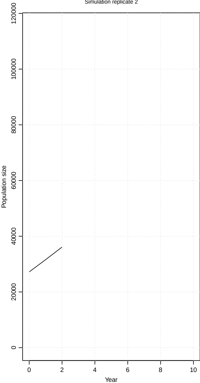
Simulation replicate 2
