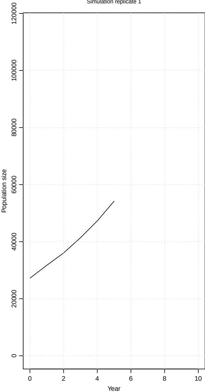
Simulation replicate 1
