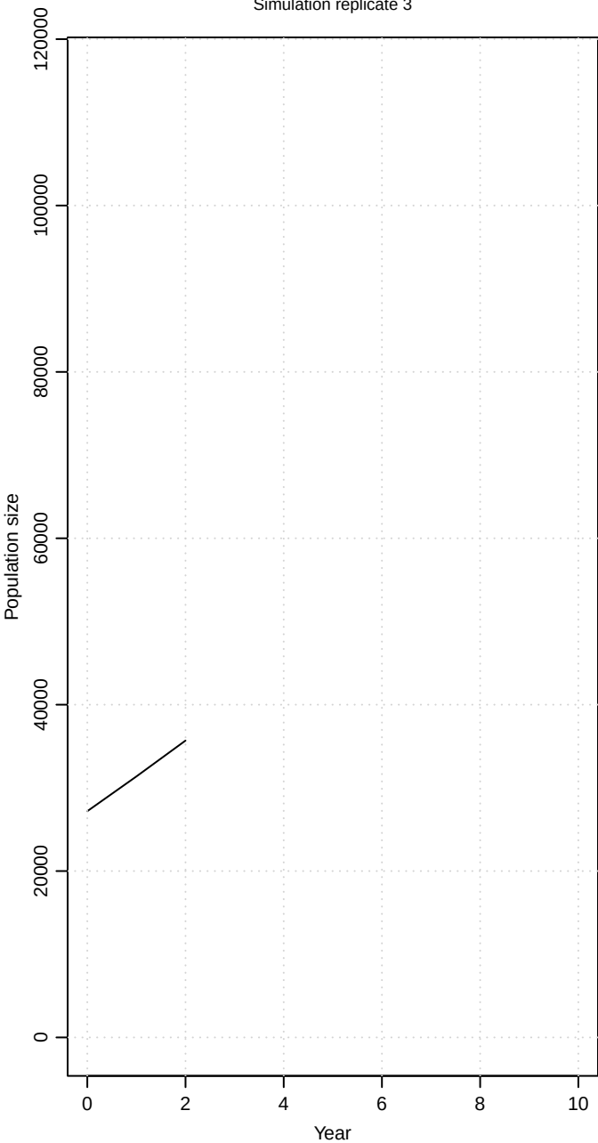
Simulation replicate 3
