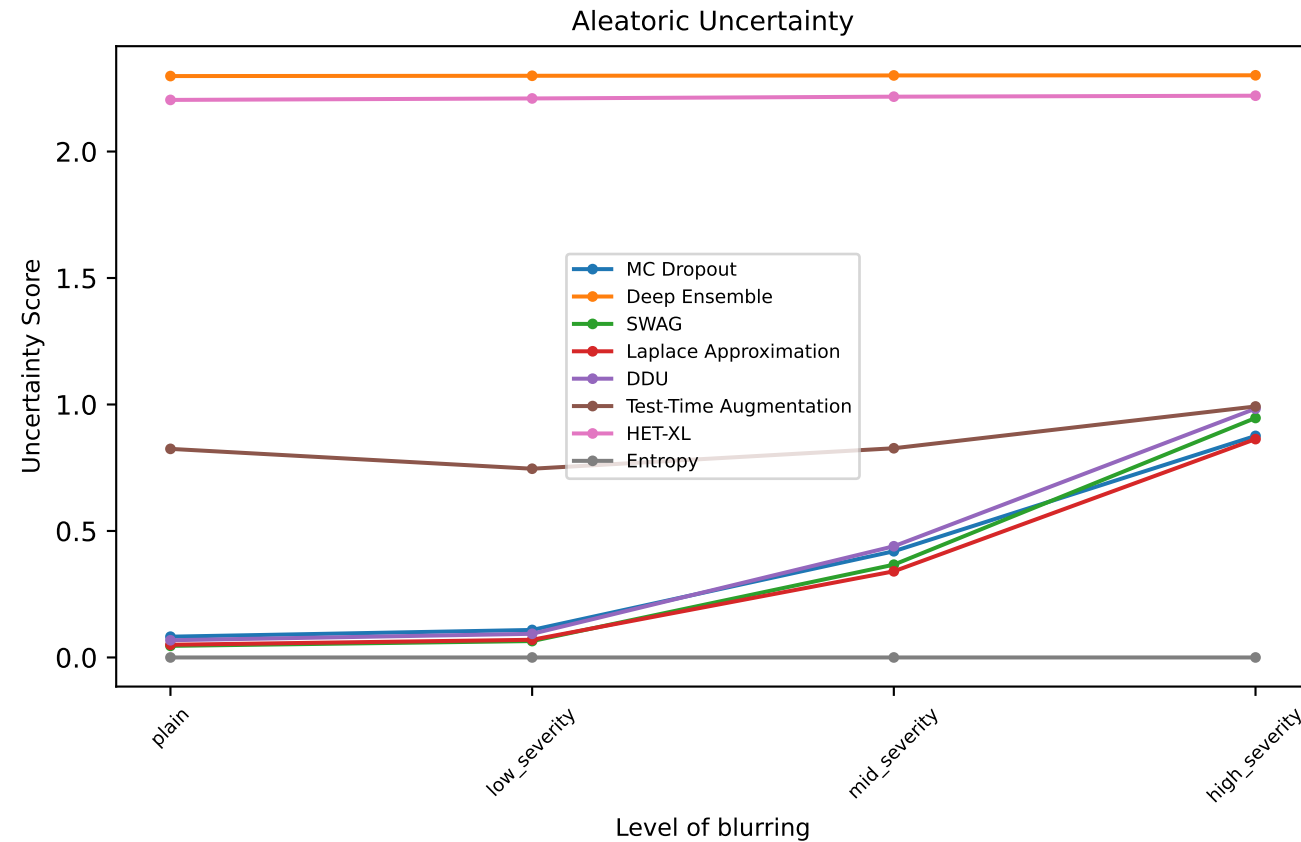
mnist_blur — all methods combined
