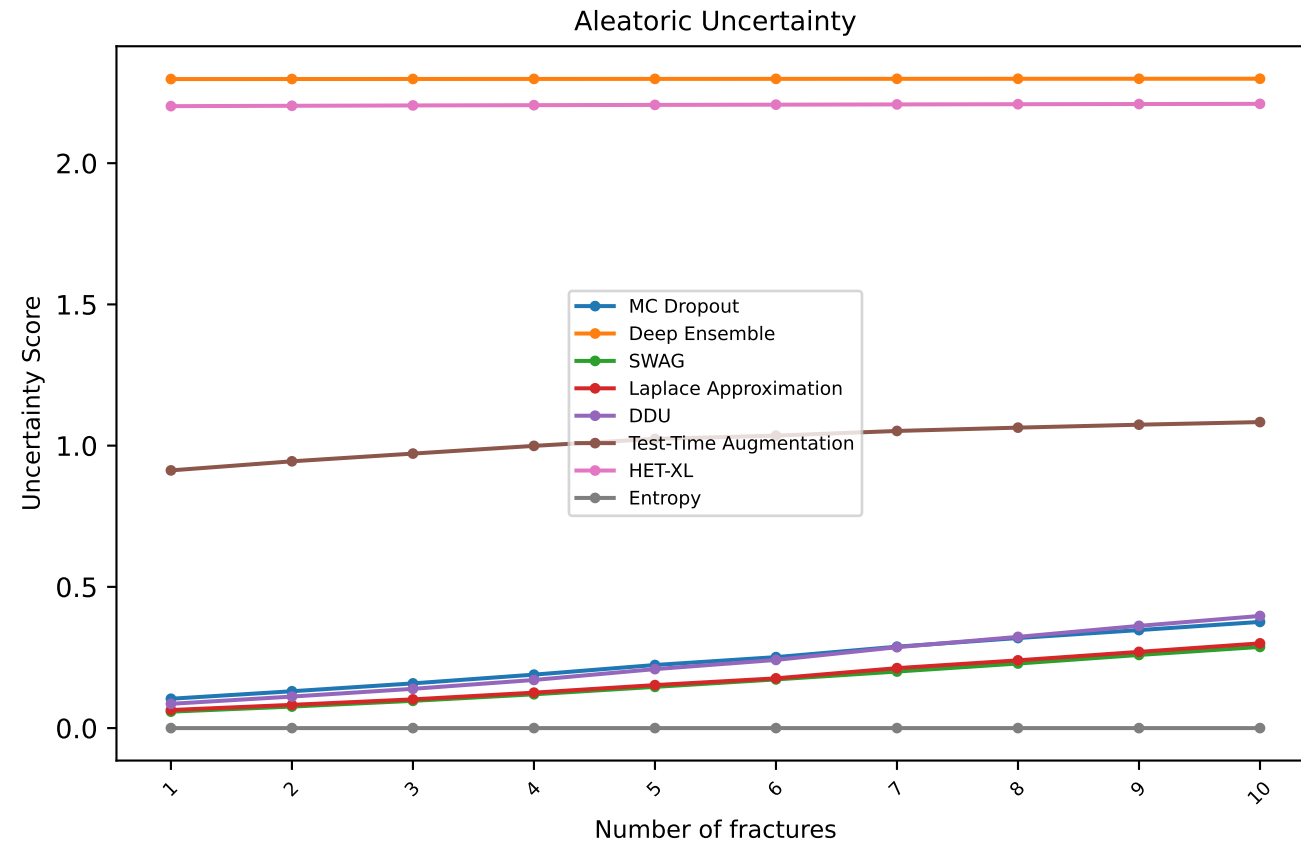
mnist_fracture — all methods combined
