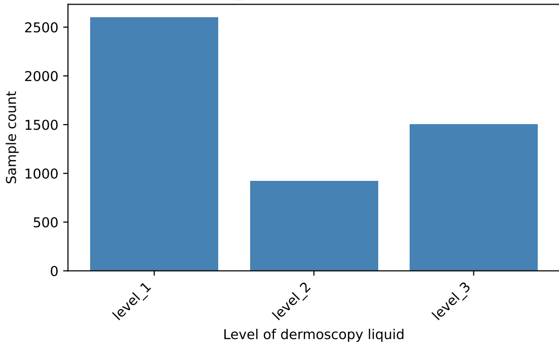
isic_drop — Distributions
