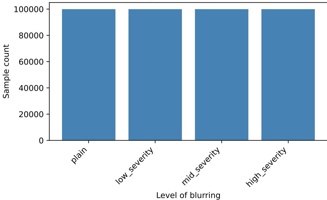
mnist_blur — Distributions
