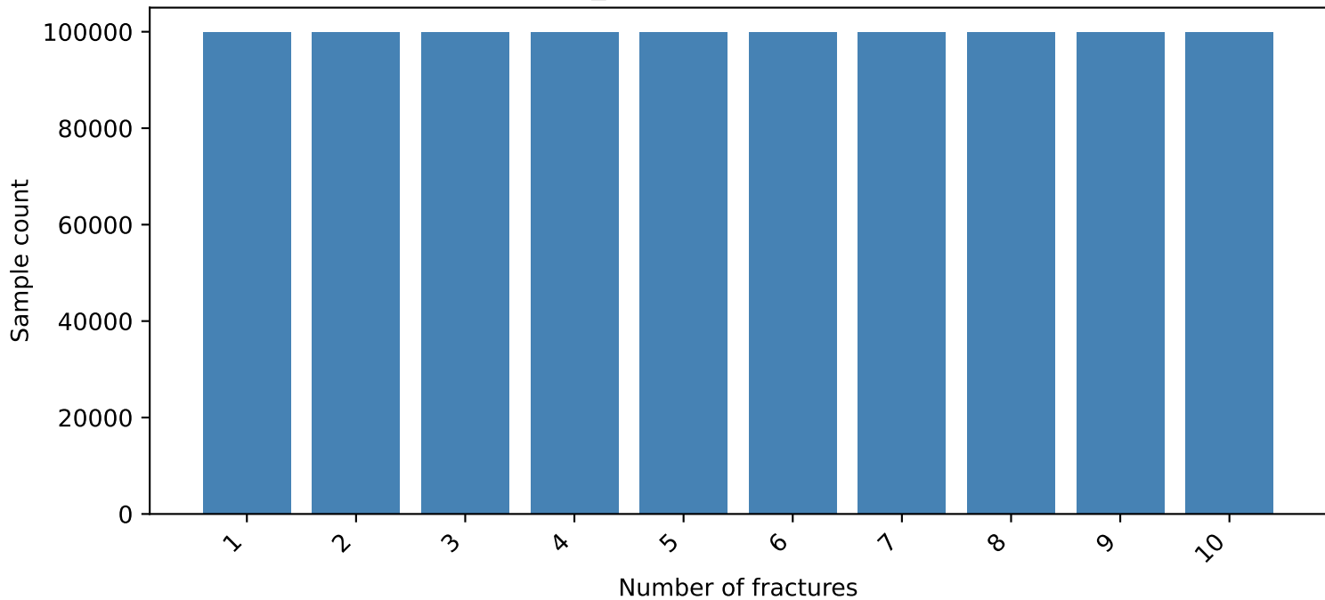
mnist_fracture — Distributions
