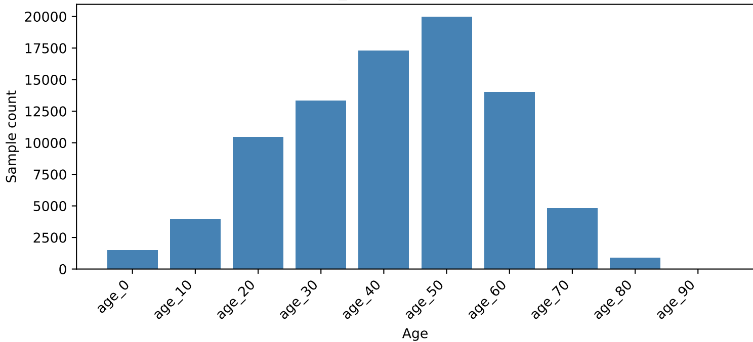
nih_age — Distributions
