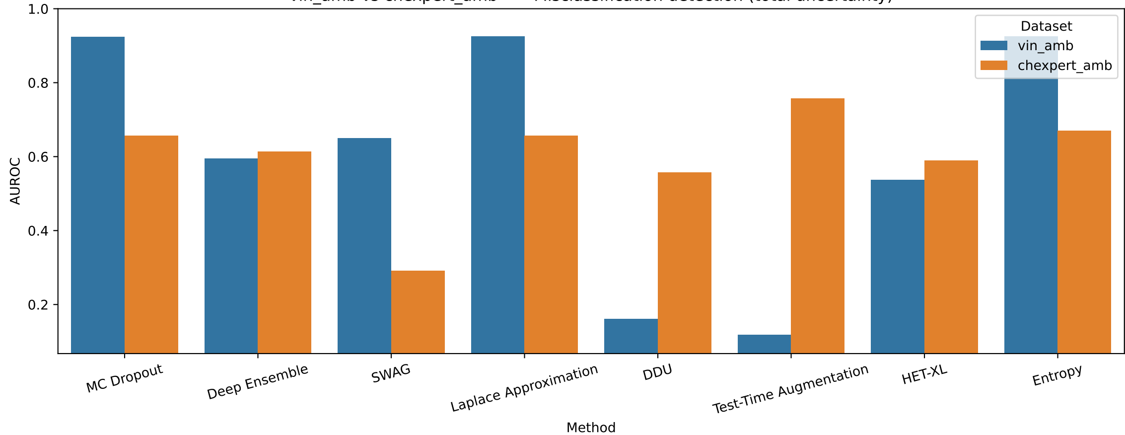
vin_amb vs chexpert_amb — Misclassification detection (total uncertainty)
