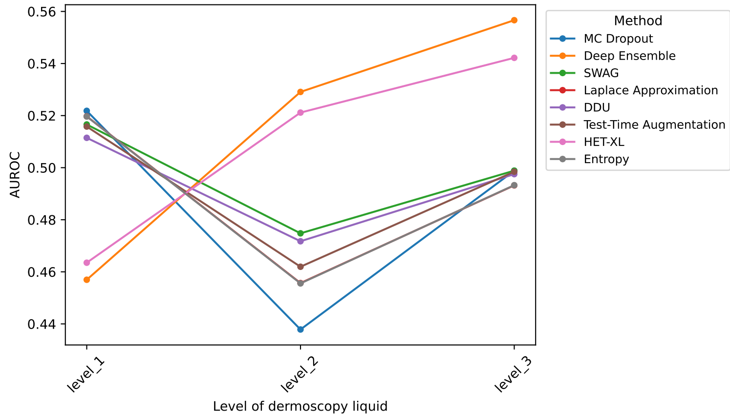
isic_drop — OOD AUROC (total uncertainty)
