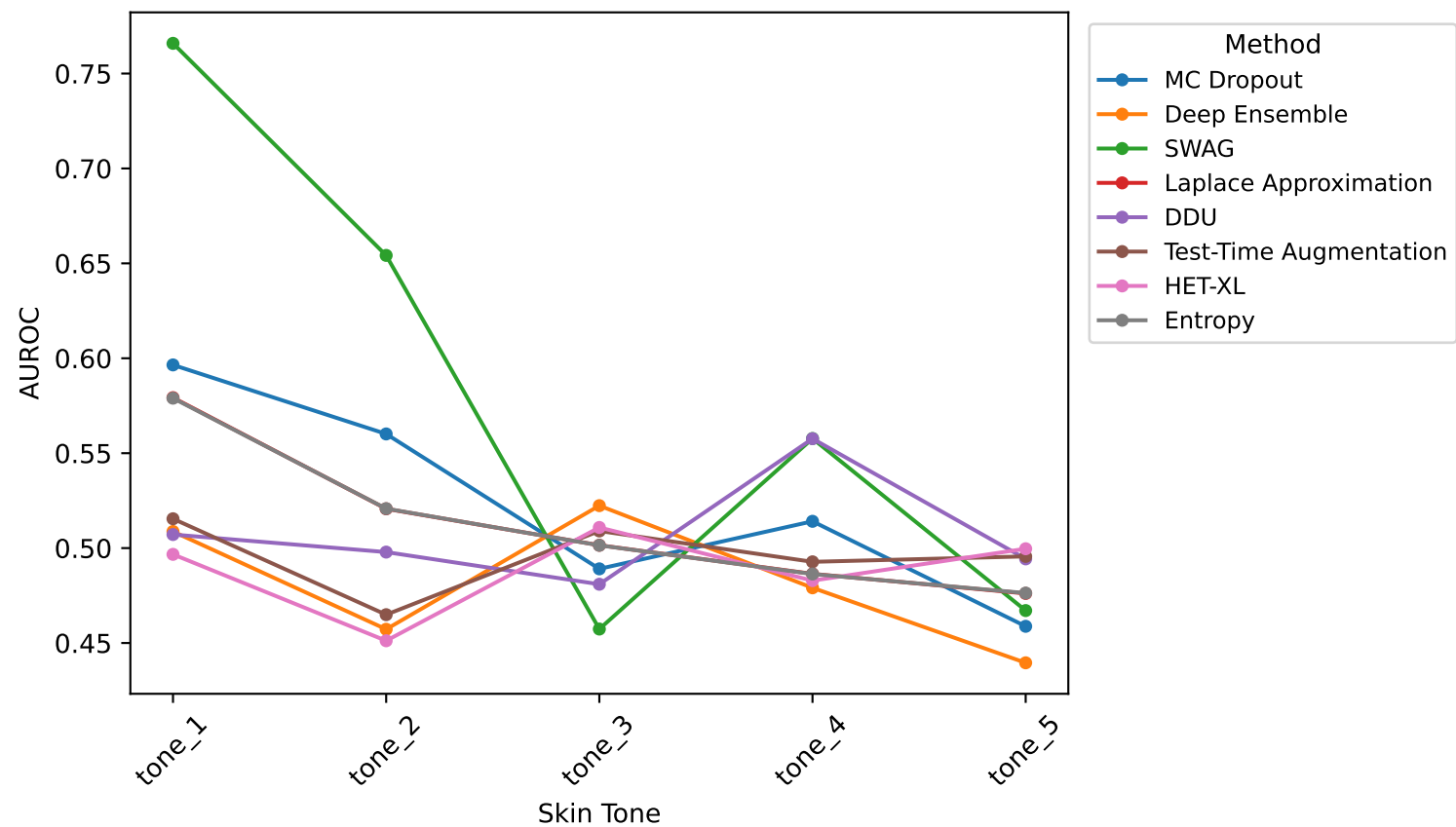
isic_skin_tone — OOD AUROC (total uncertainty)
