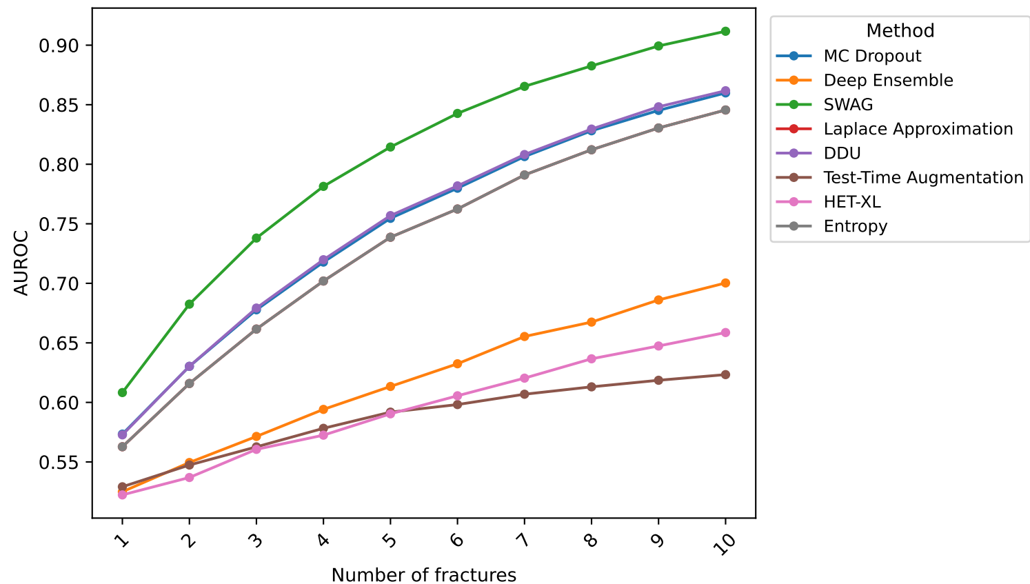
mnist_fracture — OOD AUROC (total uncertainty)
