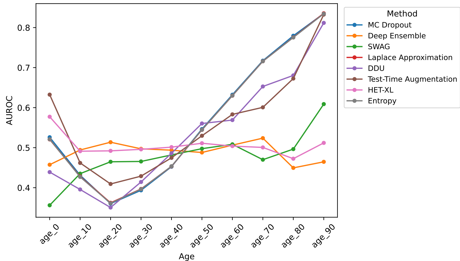
nih_age — OOD AUROC (total uncertainty)
