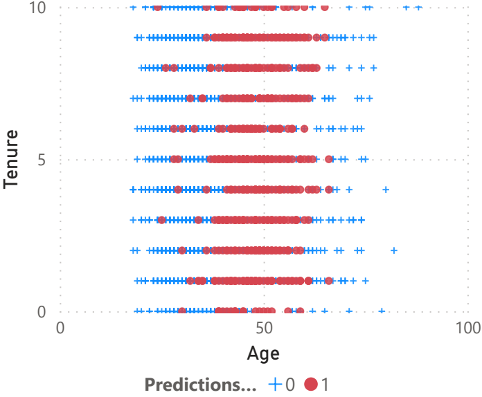
Age VS Tenure
