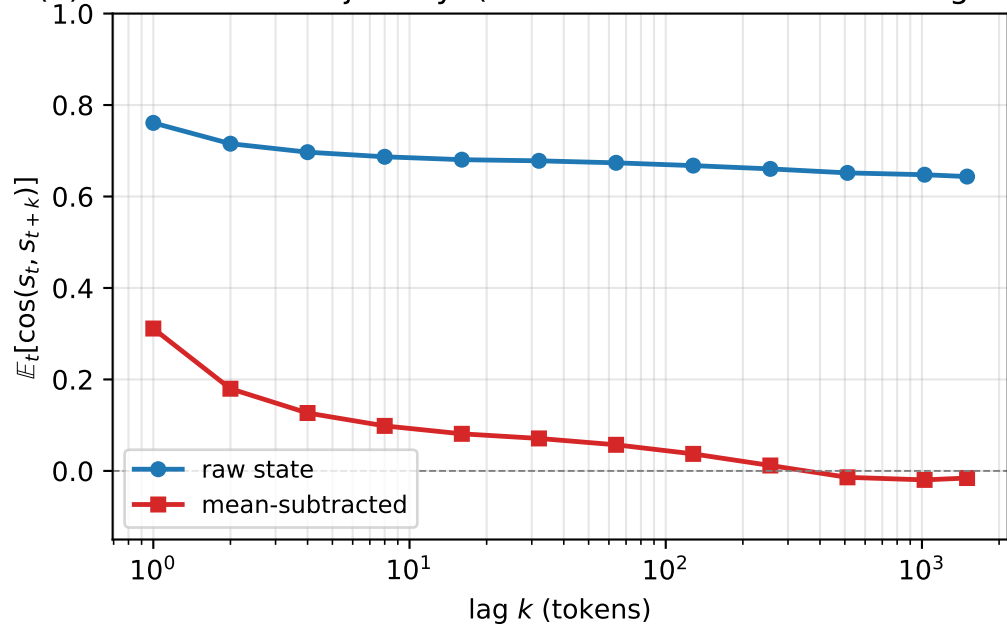
(a) State cosine trajectory (mean direction = 58% of magnitude)
