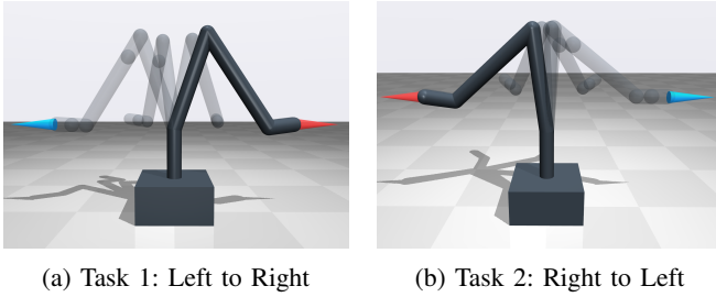
Fig. 6: Side-to-Side outreach evaluation. The manipulator navigates from the start pose (blue marker) to the goal pose (red marker) across the workspace. Faded models illustrate the intermediate trajectory states discovered by RRT-Connect. This task evaluates the morphology’s ability to maximize lateral reach and avoid collision with its own base.
