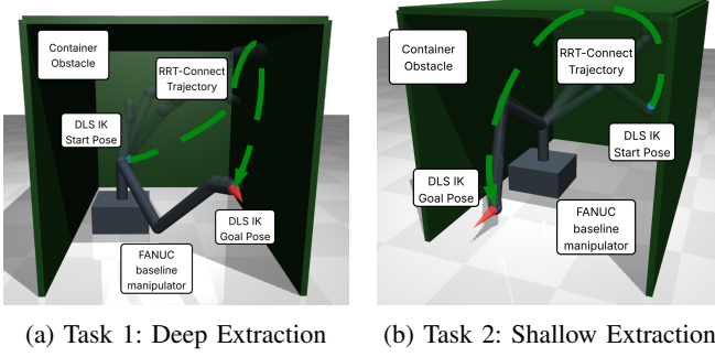
Fig. 2: Container task evaluation. The manipulator is tasked with reaching deep into a constrained, container-like environment (start poses in blue) and extracting to an open area (goal poses in red). This highly constrained task tests the morphology’s compactness and ability to perform high-reach tasks without colliding with ceiling or wall constraints.
