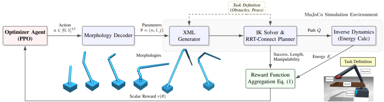
Figure 1: System overview of the proposed morphology optimization framework. The PPO agent generates actions a \in [0, 1]^{15} , which are decoded into robot parameters \theta = (n, l, j) (number of links, lengths, and joint types). These are used to create an XML model evaluated in a MuJoCo simulation environment, incorporating task definitions (obstacles and start/goal poses). IK solving and RRT-Connect path planning compute trajectories Q , followed by inverse dynamics for energy E . Performance metrics (success, path length, manipulability, and energy) are aggregated via the reward function in Eq. (1) to yield a scalar reward r(\theta) .
