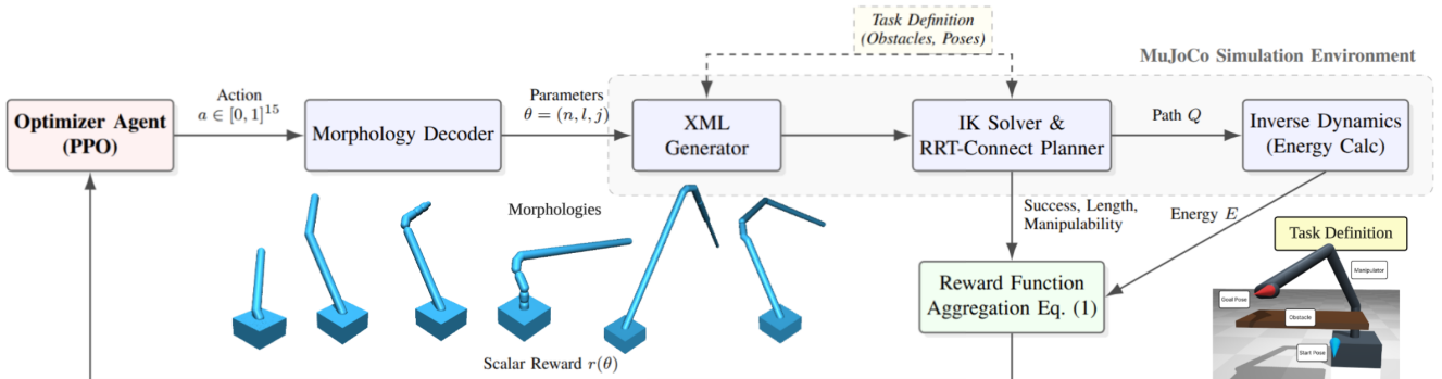
Fig. 1: System overview of the proposed morphology optimization framework. The PPO agent generates actions a \in [0, 1]^{15} , which are decoded into robot parameters \theta = (n, l, j) (number of links, lengths, and joint types). These are used to create an XML model evaluated in a MuJoCo simulation environment, incorporating task definitions (obstacles and start/goal poses). IK solving and RRT-Connect path planning compute trajectories Q , followed by inverse dynamics for energy E . Performance metrics (success, path length, manipulability, and energy) are aggregated via the reward function in Eq. (1) to yield a scalar reward r(\theta) .
