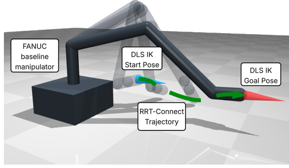
Fig. 5: Near-Base Outreach task evaluation. The manipulator extends from a configuration near its base (blue marker) to a distant target coordinate (red marker). Transparent overlays depict the collision-free joint-space trajectory generated by RRT-Connect, terminating at the opaque goal configuration. This obstacle-free environment specifically isolates and evaluates a morphology’s maximum functional reach and extension efficiency.
