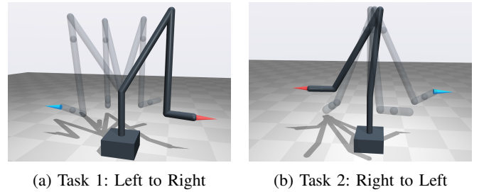
Fig. 5: Side-to-Side outreach evaluation. The manipulator navigates from the start pose (blue marker) to the goal pose (red marker) across the workspace. Faded models illustrate the intermediate trajectory states discovered by RRT-Connect. This task evaluates the morphology’s ability to maximize lateral reach and avoid collision with its own base.
