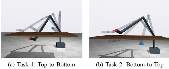
Fig. 3: Shelf task evaluation. The manipulator navigates around a floating shelf obstacle, moving from a start pose (blue marker) to a goal pose (red marker). Transparent models illustrate the intermediate joint-space trajectory, concluding at the opaque target configuration. This task specifically tests the morphology’s capability to maneuver through vertically constrained spaces and perform complex over-and-under reaching motions typical in industrial pick-and-place operations.
