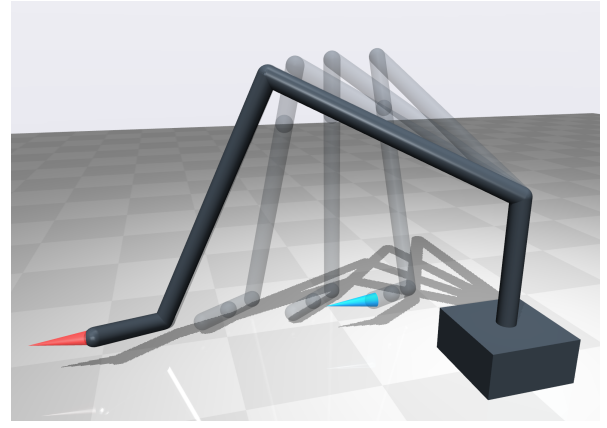
Fig. 4: Near-Base Outreach task evaluation. The manipulator extends from a configuration near its base (blue marker) to a distant target coordinate (red marker). Transparent overlays depict the collision-free joint-space trajectory generated by RRT-Connect, terminating at the opaque goal configuration. This obstacle-free environment specifically isolates and evaluates a morphology’s maximum functional reach and extension efficiency.
