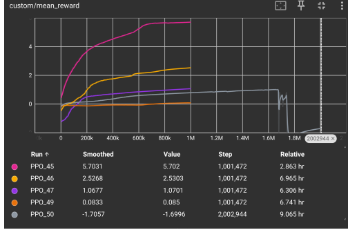
Fig. 7. Rewards per Episode Plot
