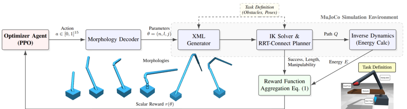
Fig. 1: System overview of the proposed morphology optimization framework. The PPO agent generates actions a \in [0, 1]^{15} , which are decoded into robot parameters \theta = (n, l, j) (number of links, lengths, and joint types). These are used to create an XML model evaluated in a MuJoCo simulation environment, incorporating task definitions (obstacles and start/goal poses). IK solving and RRT-Connect path planning compute trajectories Q , followed by inverse dynamics for energy E . Performance metrics (success, path length, manipulability, and energy) are aggregated via the reward function in Eq. (1) to yield a scalar reward r(\theta) .
