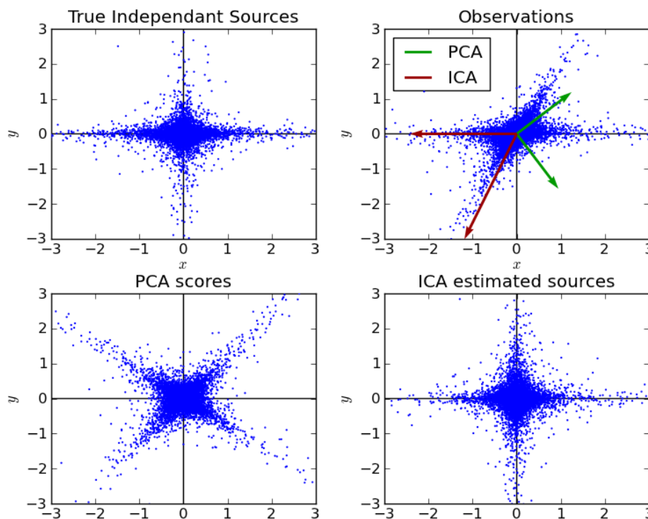
Figure 4.2: PCA decorrelates the observations but does not recover the independent axes. ICA uses higher-order structure to rotate the representation back towards the true independent sources.
