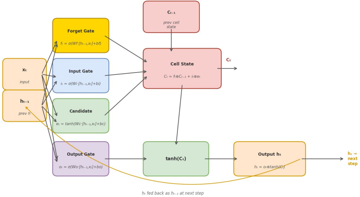
Figure 9. LSTM Architecture.
