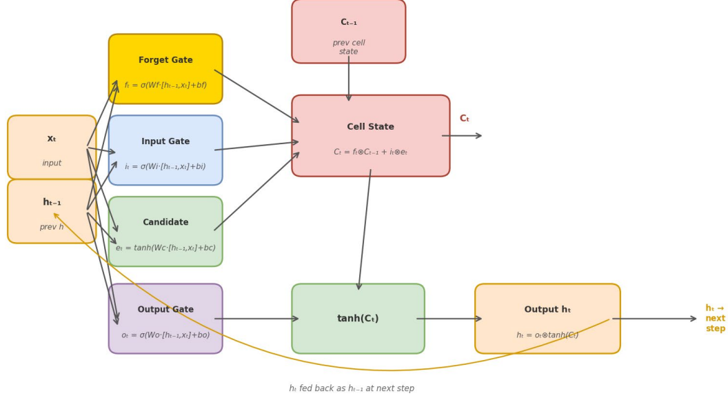
Figure 9. LSTM Architecture.
