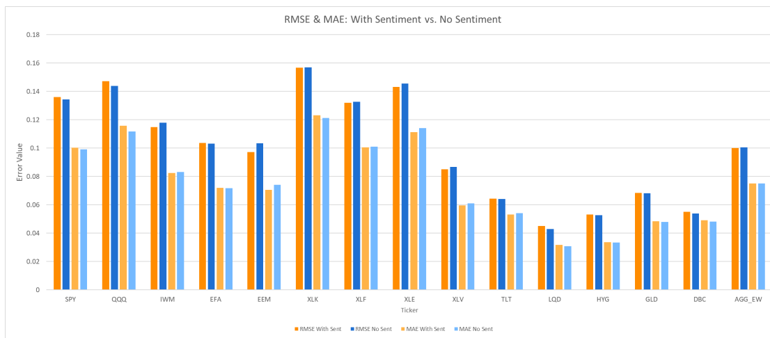
Figure 16. RMSE and MAE Bar Plot of XGBoost without Sentiment and XGBoost with Sentiment.
