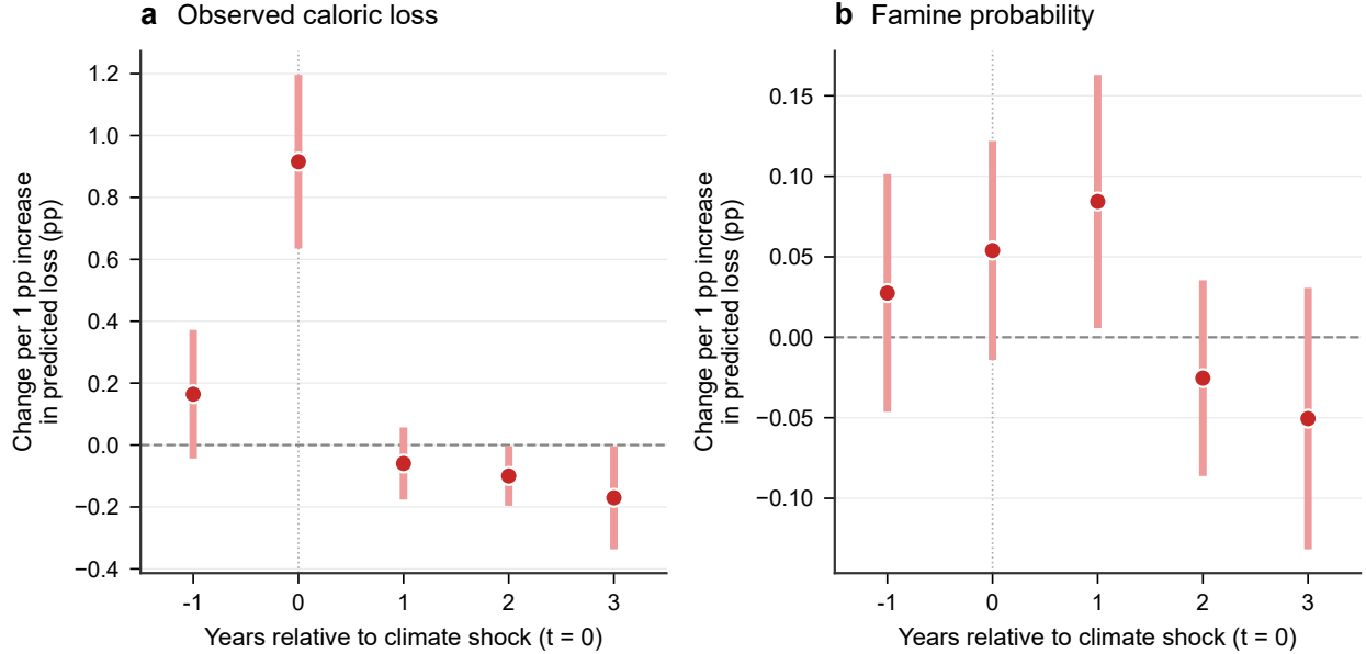
Figure 3: Agricultural losses coincide with climate shocks and famine risk rises subsequently. Distributed-lag coefficients for observed caloric production loss (a) and famine-year probability (b), per one-percentage-point increase in predicted production loss by the temperature-soil moisture model. The plotted window includes one year before the shock, the shock year and three subsequent years. Shading denotes 95% confidence intervals.
