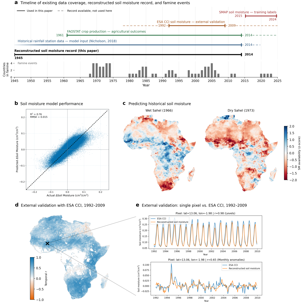
Figure 1: Reconstructing historical soil moisture across Africa. a , Coverage of the reconstruction, input and comparison datasets, and coded famine years. Dashed intervals indicate available records outside the windows used. b , Predicted versus observed monthly soil moisture changes in the withheld modern SMAP L4 test split ( R^2 = 0.76 ; \text{RMSE} = 0.015 \text{ cm}^3 \text{ cm}^{-3} ). c , Standardized reconstructed moisture availability across Africa in 1966 and 1973. d , Pixel-wise temporal correlation with ESA CCI during 1992–2009 after removing grid-cell-specific monthly climatologies. Missing data in ESA CCI due to dense vegetation cover is masked out. e , Levels and deseasonalized anomalies at a location in Sahel.
