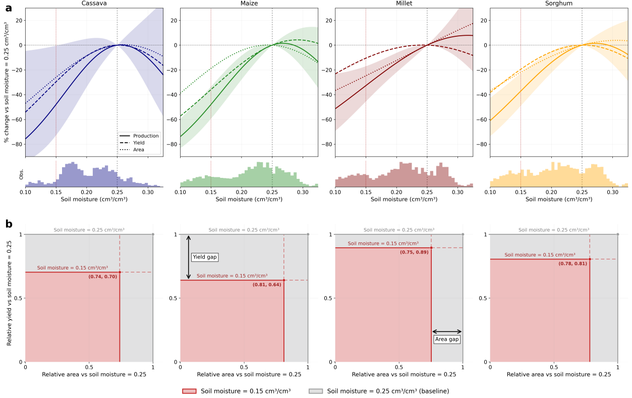
Figure 2: Harvested-area losses amplify the agricultural response to dry soils. a , Crop-specific production, yield and harvested-area responses to soil moisture in quadratic temperature–soil moisture models. Responses are normalized to 0.25 cm³ cm⁻³; shading shows 95% confidence intervals for production. Histograms show moisture support in the plotting sample. Regressions include country–crop fixed effects and country trends, with country–crop-clustered standard errors. b , Yield and area ratios at 0.15 relative to 0.25 cm³ cm⁻³. Rectangle width is relative harvested area, height is relative yield and their product is relative production; labels give (relative area, relative yield) at 0.15 cm³ cm⁻³.
