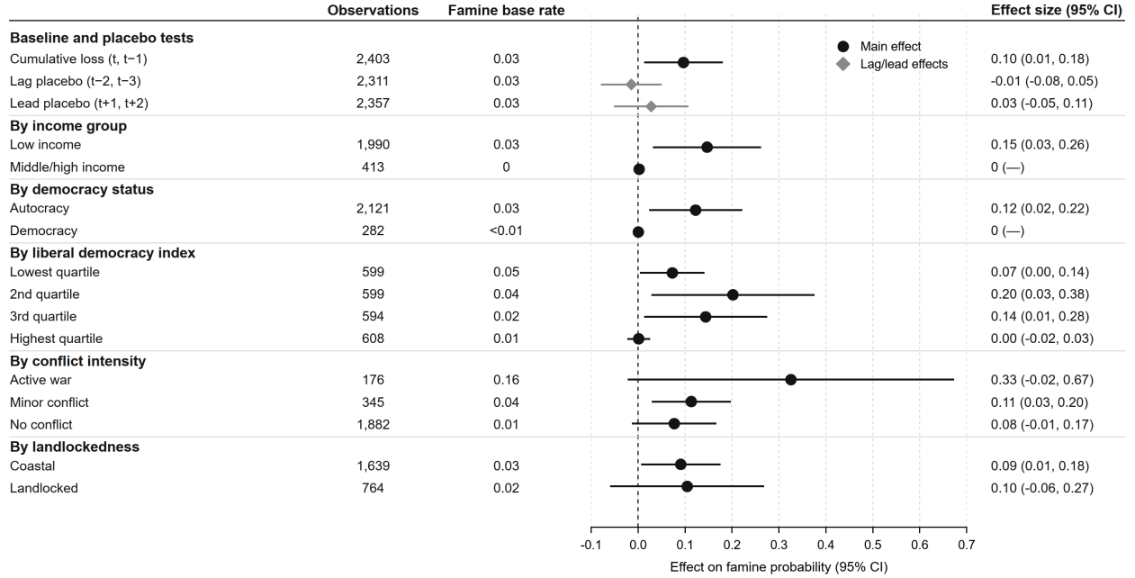
Figure 5: The loss–famine relationship varies across economic and political settings. Baseline and displaced-window estimates represent separate country–decade fixed-effects regressions. Heterogeneity rows use interaction models, with subgroup slopes recovered by linear combinations and standard errors clustered by country. Exposure is the sum of current and previous annual losses, in fractional units. Multiplying a reported slope by 10 gives the percentage-point probability change for a ten-percentage-point increase in summed loss. Columns report subgroup observations, famine base rates and 95% confidence intervals.
