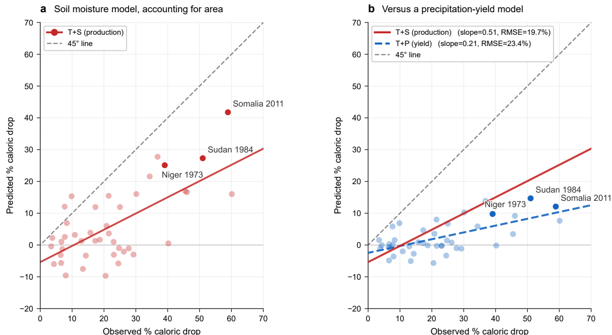
Figure 4: Soil moisture and harvested area improve the prediction of famine-year shortfalls. Observed and out-of-sample predicted caloric production losses in the 42 famine country-years with observed caloric shortfalls. Each prediction comes from models estimated without that country-year. a , Temperature–soil (T+S) moisture production predictions versus a one-for-one reference line. b , Comparison with a temperature–precipitation (T+P) yield model.
