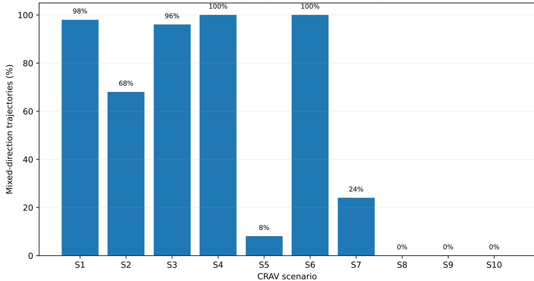
Within-trajectory directional switching
