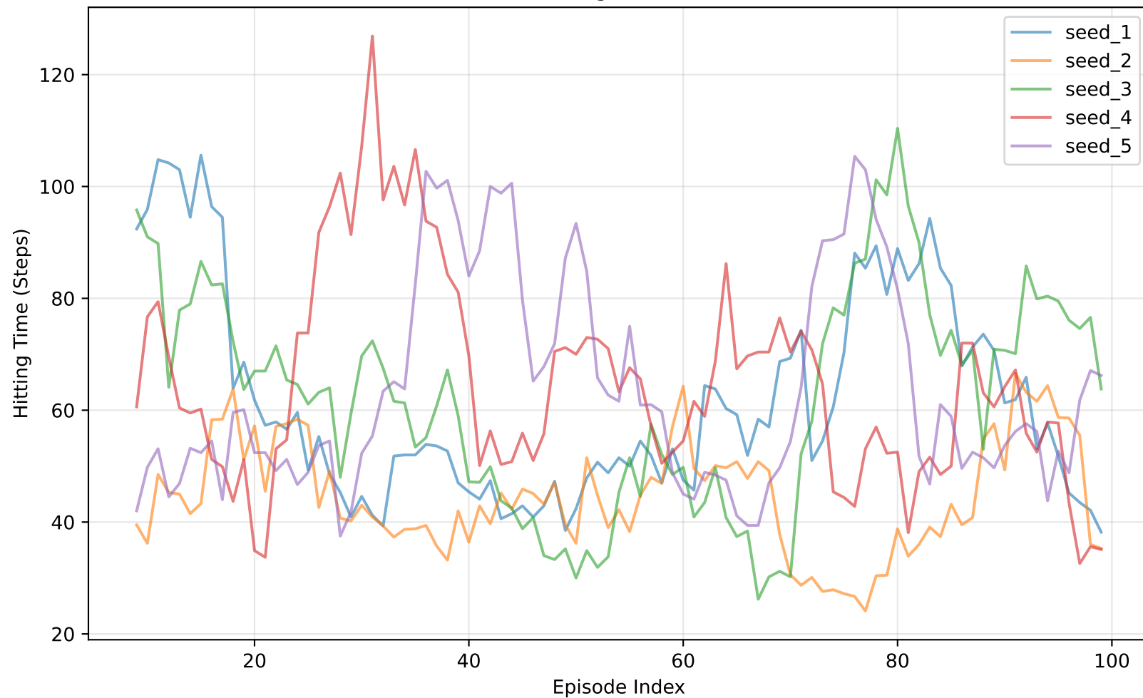
Baseline Hitting Times (Per Seed)
