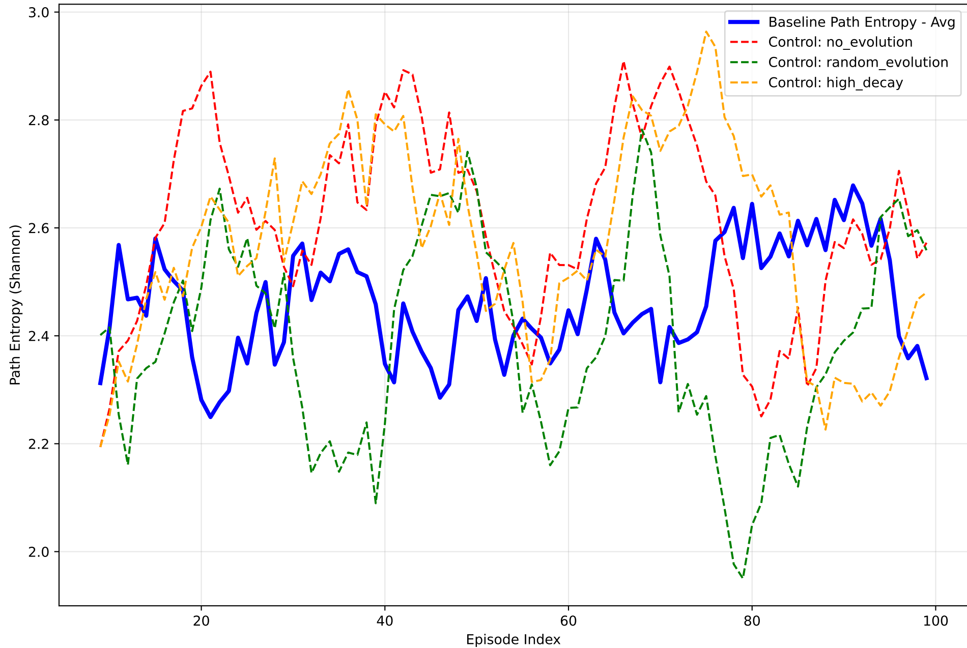
HCCDE Validation: Path Entropy Trends
