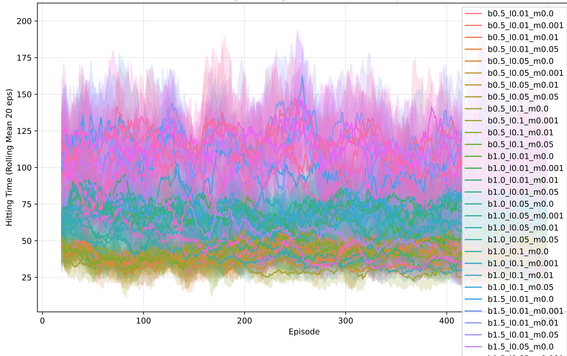
Averaged Hitting Times - Parameter map
