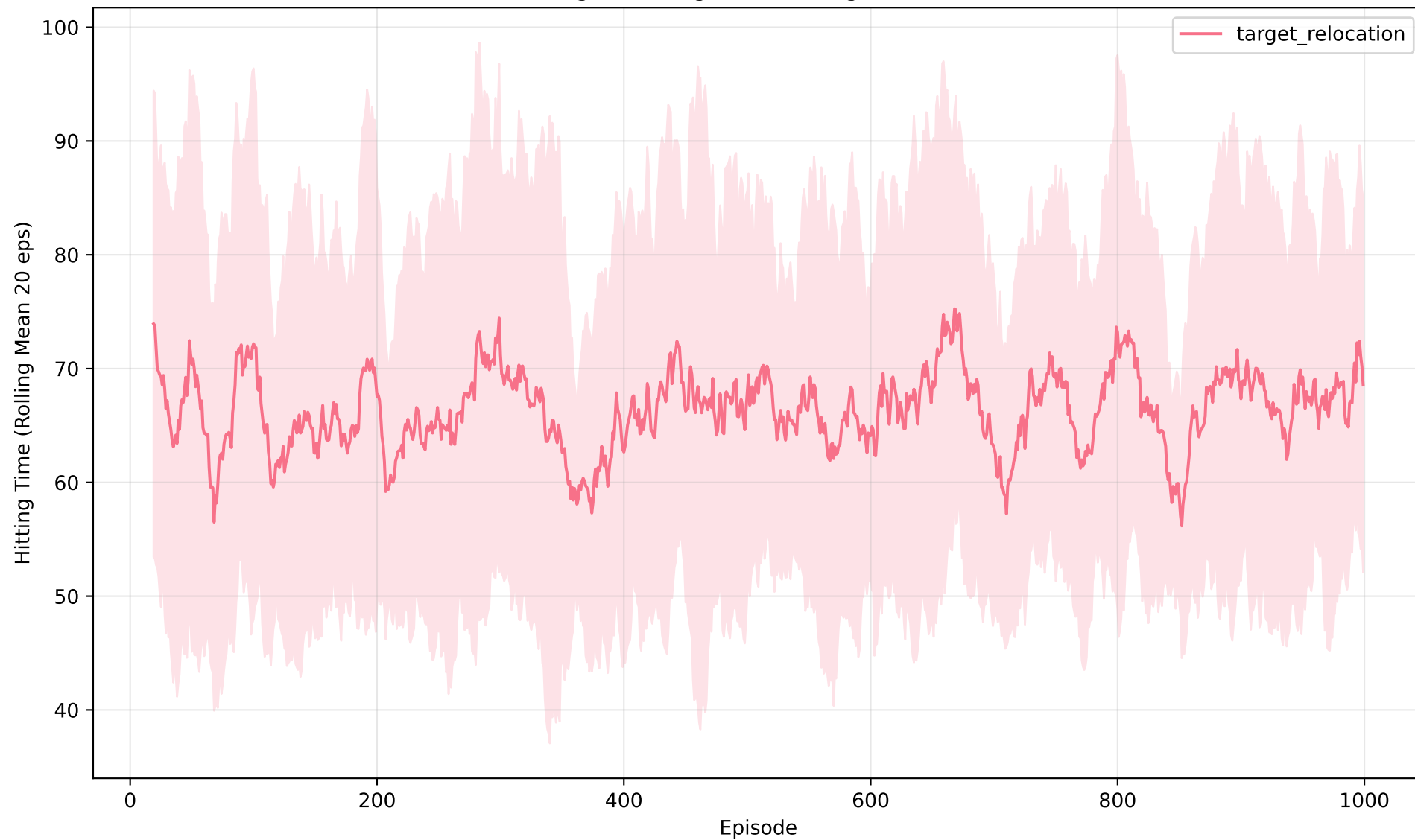
Averaged Hitting Times - Target relocation
