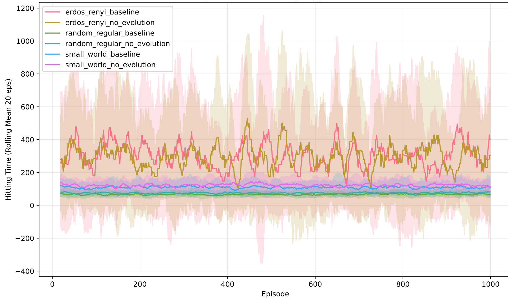
Averaged Hitting Times - Topology robustness
