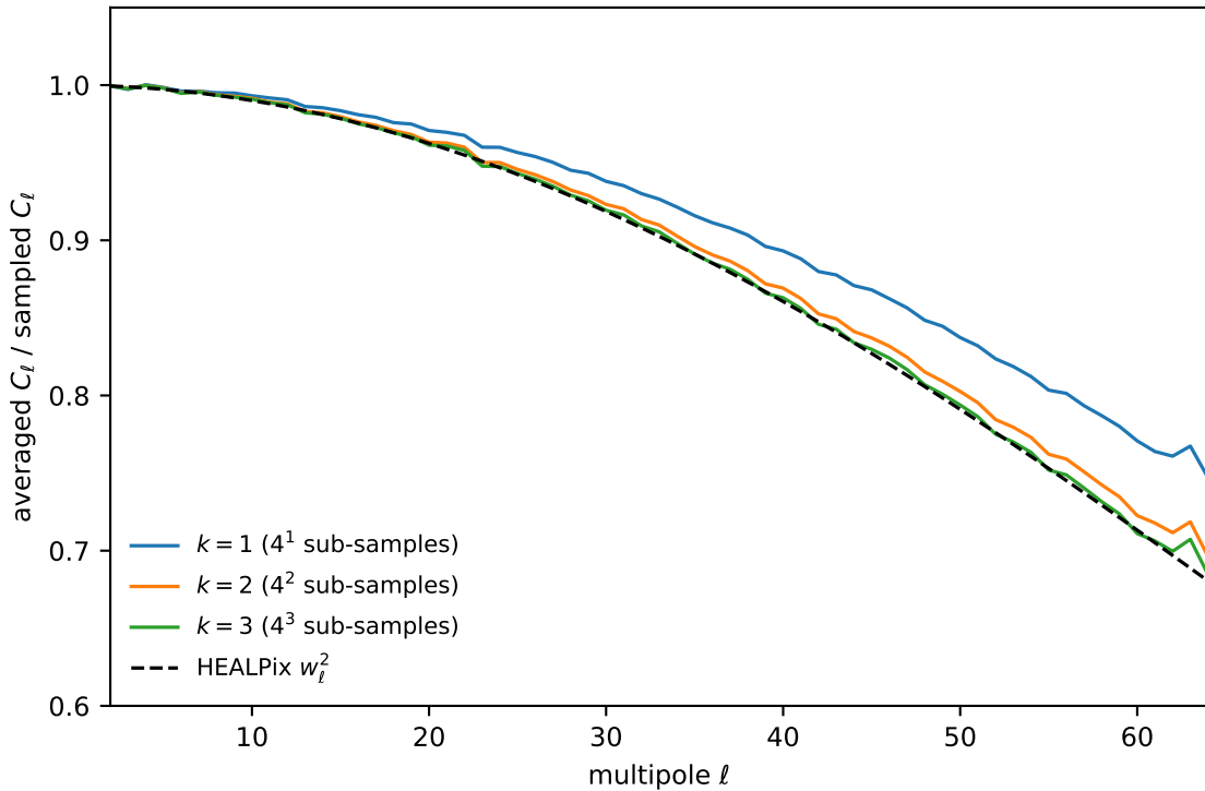
Averaging over the pixel, N_{\text{side}} = 32
