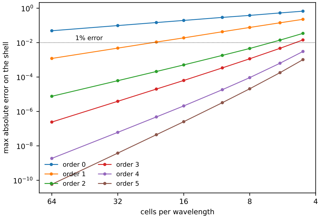
Interpolating a single Fourier mode
