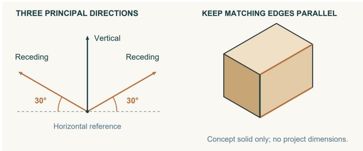
Figure 12. A generic block shows vertical edges and two receding directions at 30° to the horizontal. Edges following the same direction stay parallel.
