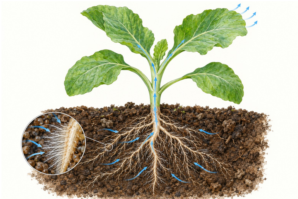
Conceptual illustration. Arrows show water uptake, upward movement and water-vapour loss. The magnified inset shows root hairs; the drawing is not to scale.
