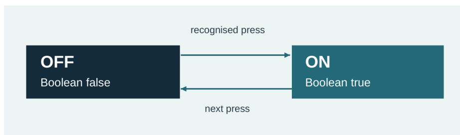
Figure 6.3. Two recognised presses invert the same stored Boolean twice.
