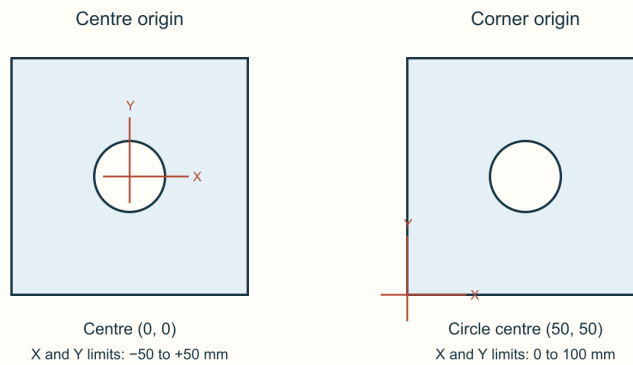
Different CAD origins, equal dimensions
