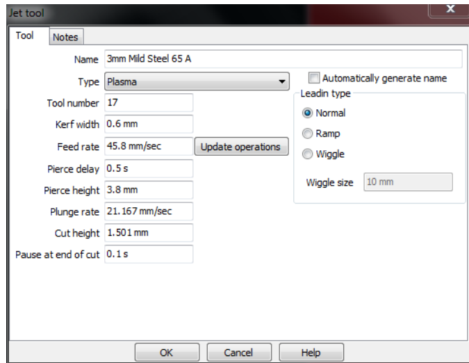
Supplier SheetCam Jet tool, SureControl manual p. 43. The feed field uses mm/sec. Confirm quantity and units before comparing any number with another screen.
