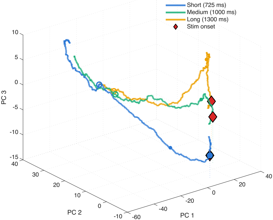
Population trajectories — stim onset aligned
