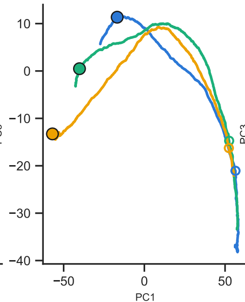
Population trajectories — PC space (stim aligned)
