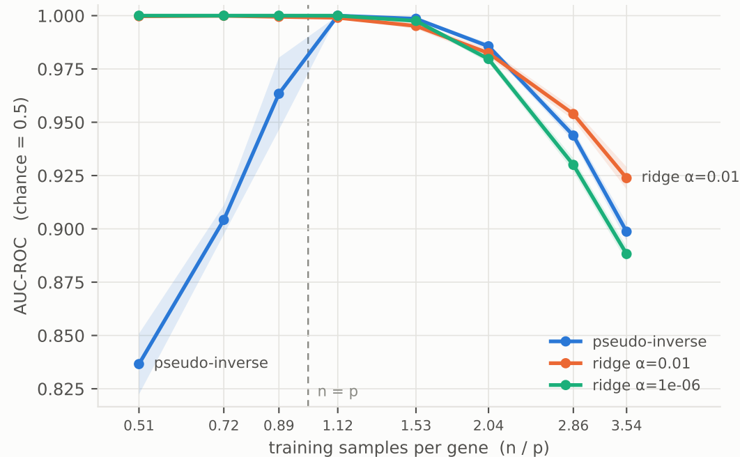
MahalaMIA vs the MVN generator, COMBINED resampled to each size
